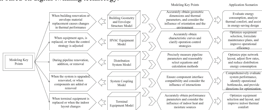
Figure 1 Digital Twin-based Air Conditioning System Model
